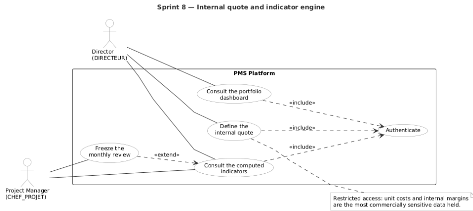
Figure 6.8: Use case diagram of sprint 8
