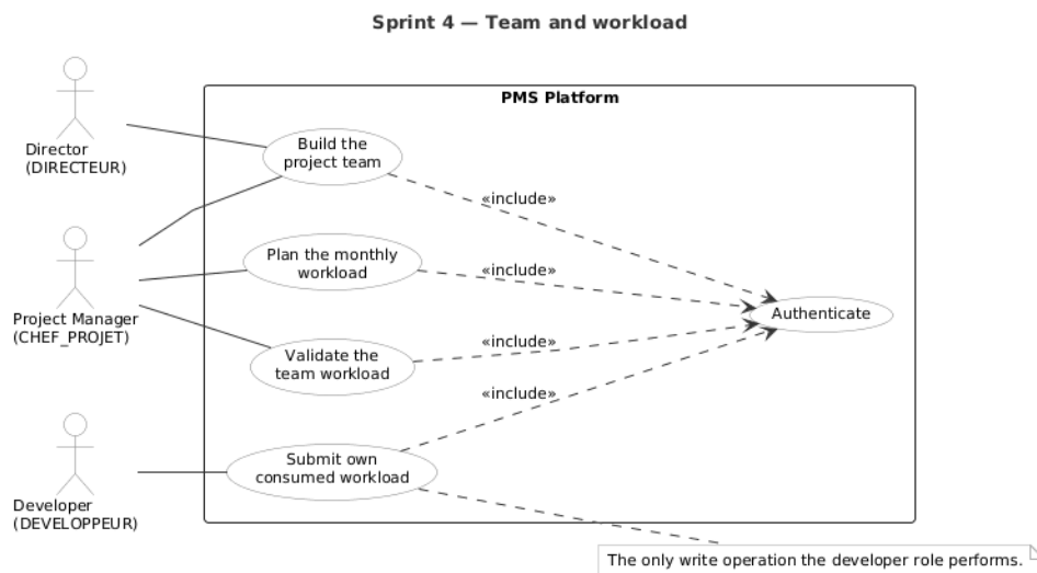
Figure 5.7: Use case diagram of sprint 4
