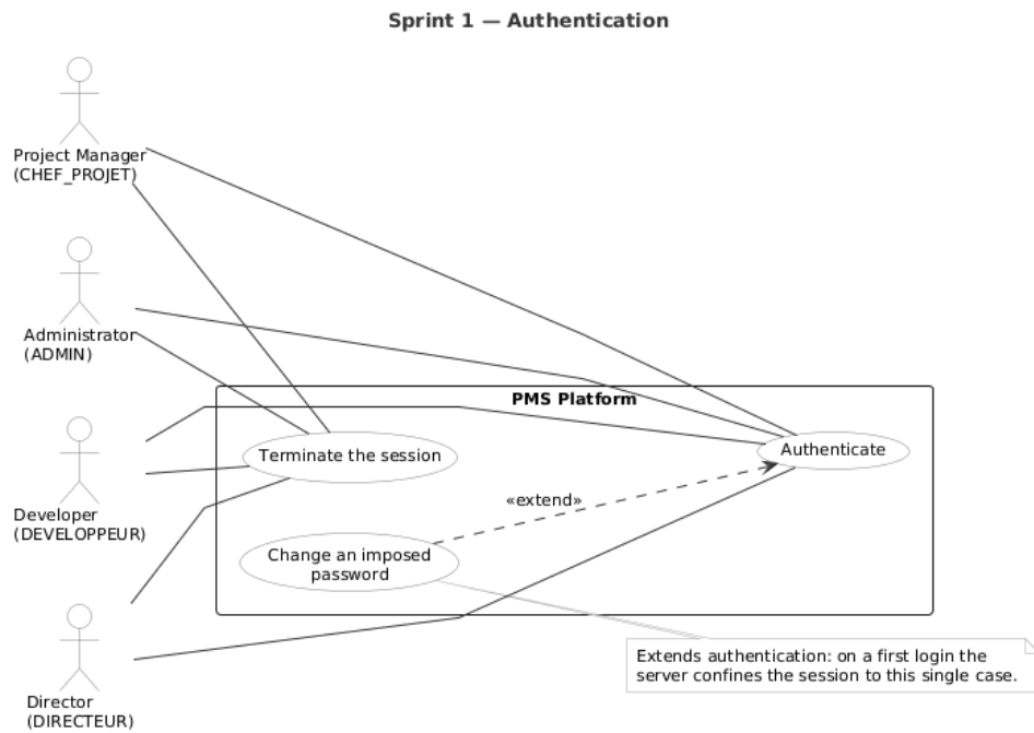
Figure 4.9: Use case diagram of sprint 1
