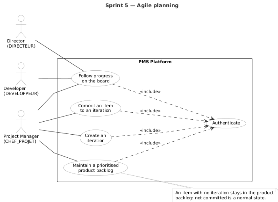
Figure 5.11: Use case diagram of sprint 5
