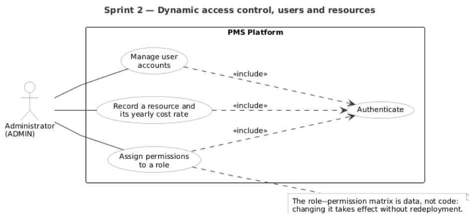
Figure 4.15: Use case diagram of sprint 2
